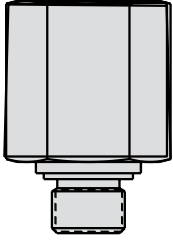
43-0000-19 转换接头, 变径, 外丝 G1/8-内丝 G1/4
