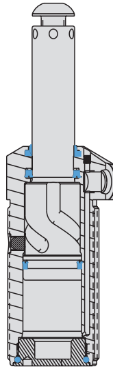
SWING CLAMP PLUNGER SHOWN IN THE EXTENDED LH CAM POSITION ILS140001 REV L
