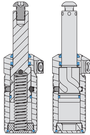
SINGLE ACTING DOUBLE ACTING SWING CLAMP PLUNGER SHOWN IN THE EXTENDED LH CAM POSITION ILS140001 REV M
