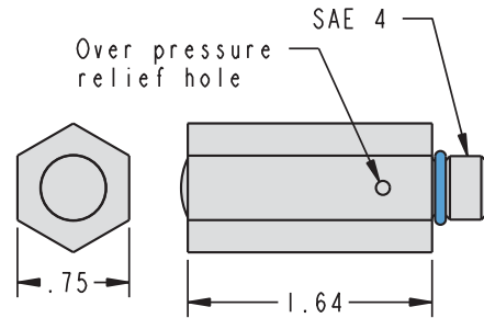
Over Pressure Relief Valve ILS706300 REV D
