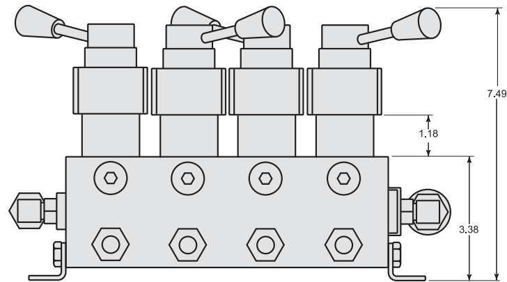
4 Valve Control Layout
