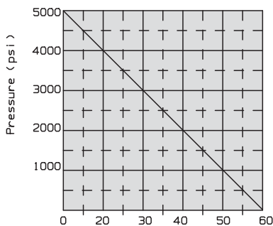
Flow rate (cu in/min) at 90 PSI Air Input ILS552001 REV D
