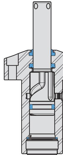
Double Acting
