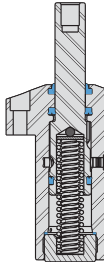
Single Acting
