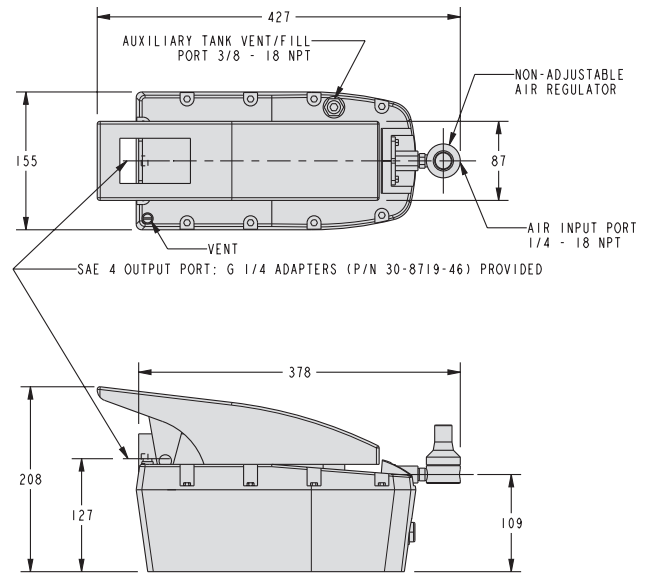
45-5820-02 MANUALLY OPERATED
