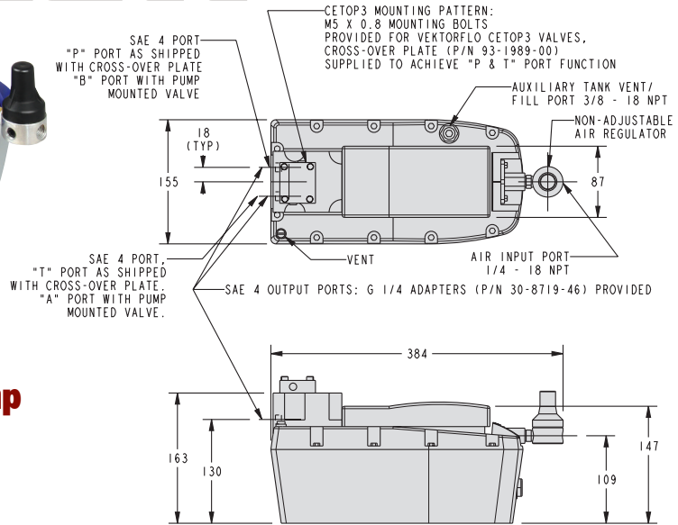
45-5820-01 VALVE MOUNTING
