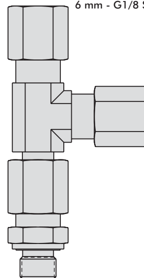
43-0000-17 Tee, Run, Swivel 6 mm - G1/8 Stud
