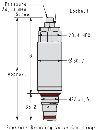
Pressure Reducing Valve Cartridge
