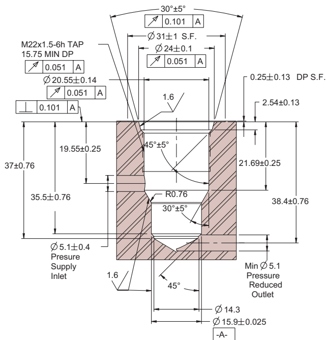
Pressure Reducing Valve Cartridge
